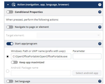
Fig. 6: Allowed applications
