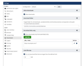
Fig. 7: Files & Downloads
